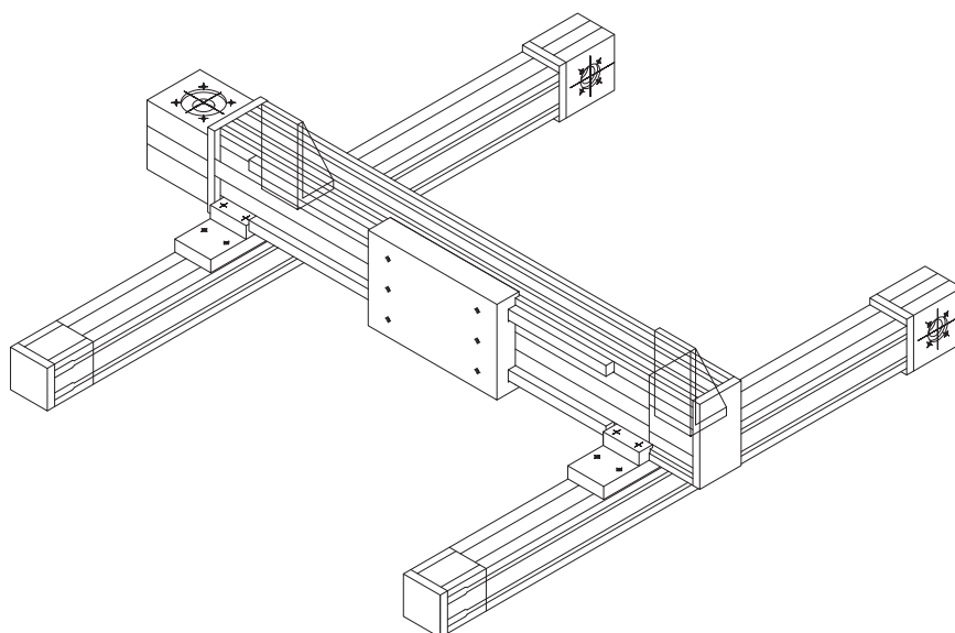
Two axis X-Y system
